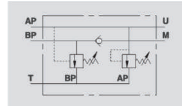
Hydraulic Symbol
