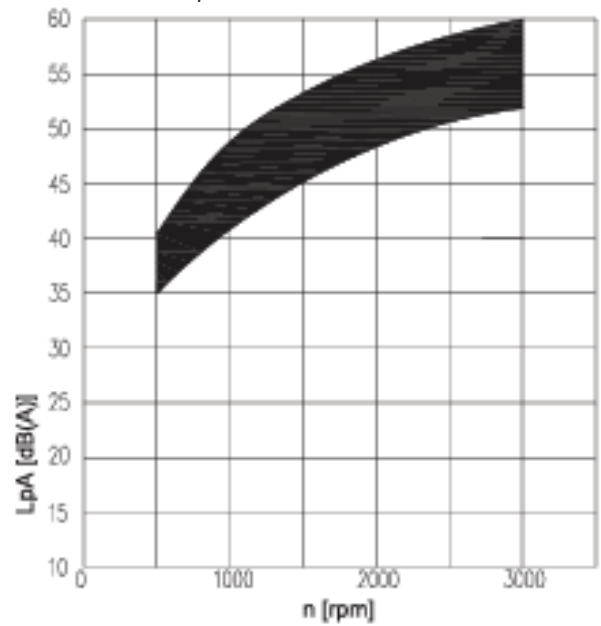
V=8.0\text{CM}^3/\text{r}
