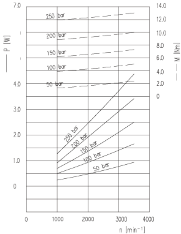
V=3.70\text{CM}^3/\text{r}
